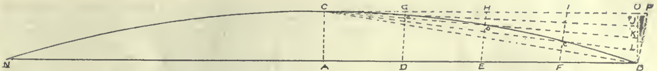
Fig. 10. Showing Method of Constructing Curve for Beams
