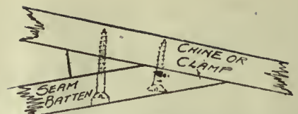
SKETCH SHOWING CONNECTION OF SEAM BATTEN TO CHINE OR CLAMP
