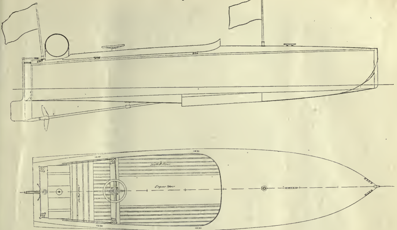
OUTBOARD PROFILE AND DECK PLAN
