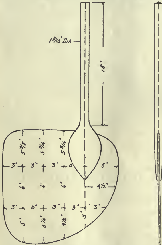
Figure 18—Balanced Rudder
