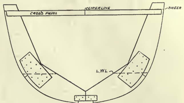
Fig. 6. Mold, Showing Cleats and Cross Pawl.
