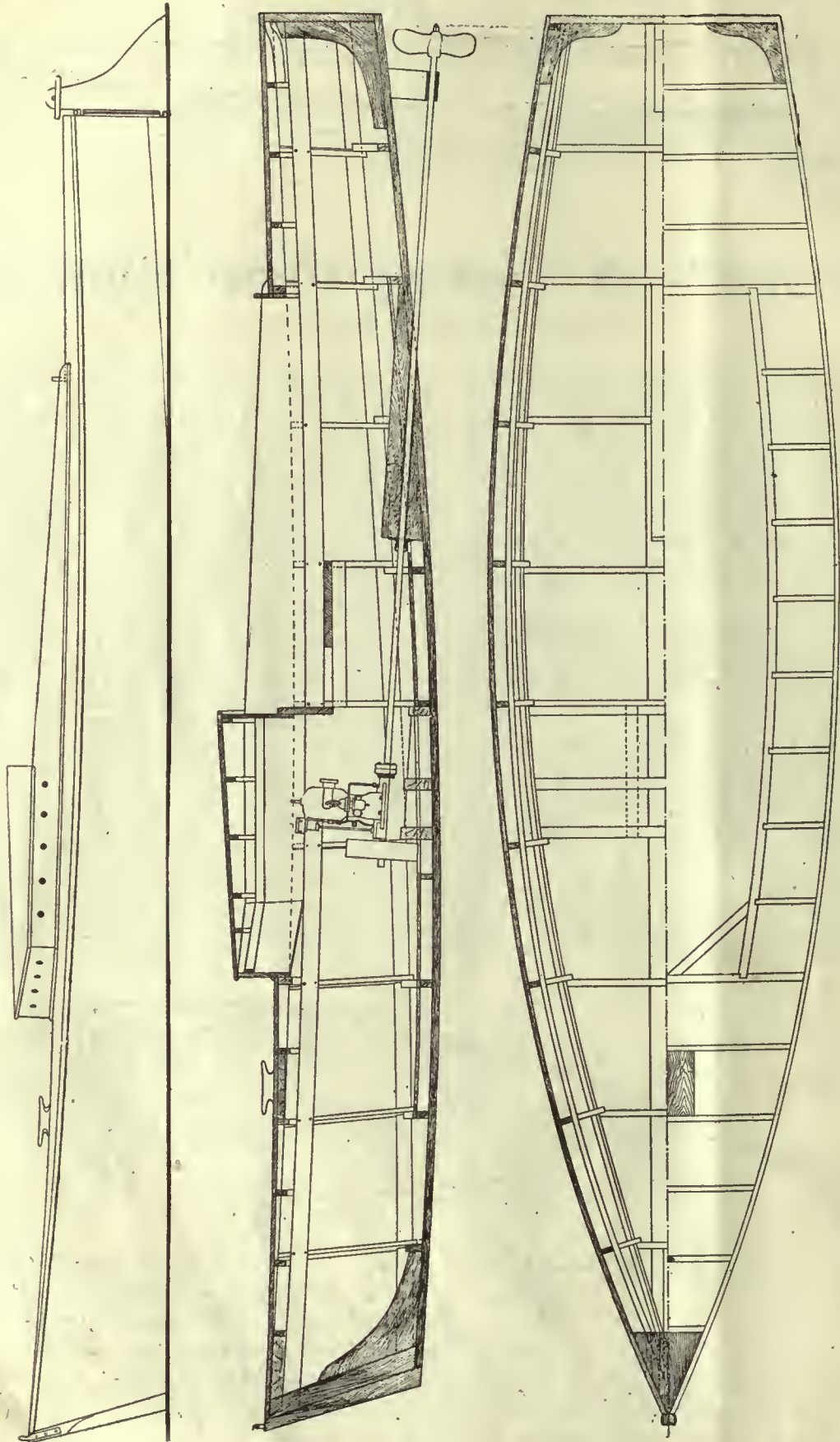
CONSTRUCTION PLANS OF "POP GUN"
