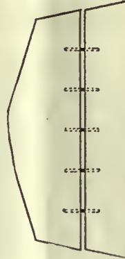
In doweling the two pieces of a transom together be sure all the dowels are parallel to each other
