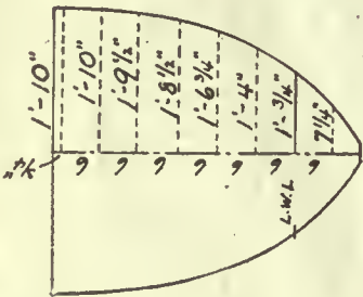
MOLD NO. 2.
