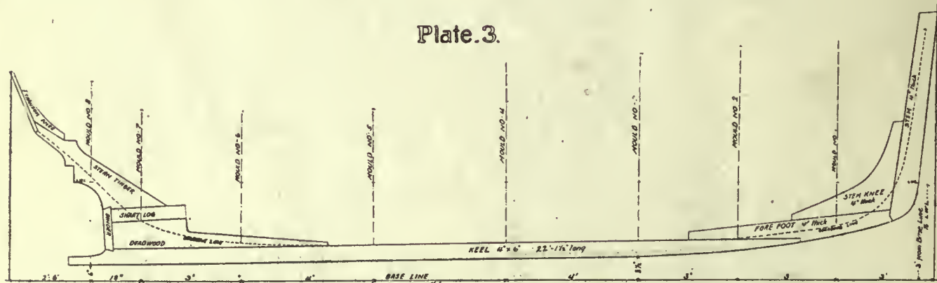
Names of the various pieces that, when all are bolted together, form the backbone of the boat's frame and the location for the various moulds.
