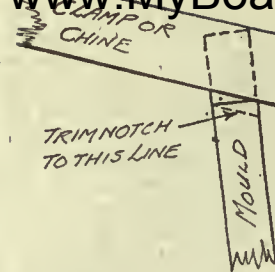
SKETCH SHOWING HOW NOTCHES IN MOLDS ARE TRIMMED TO TAKE CHINE AND CLAMP
