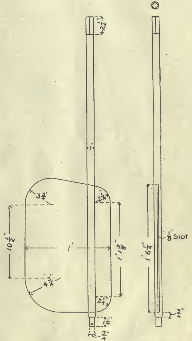
Detail Drawing of Rudder
