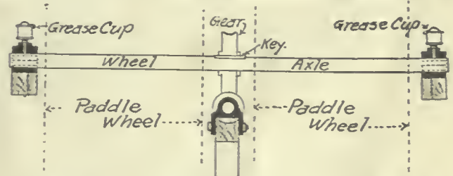
Arrangement of bearings for axle of the stern wheel and end of shaft.
