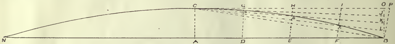
Fig. 10—Showing Method of Constructing Curve for Beams
