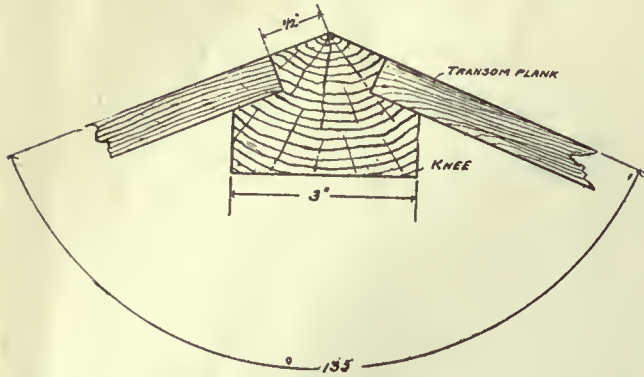
Fig. 11. Section Through Knee, Showing Angle
